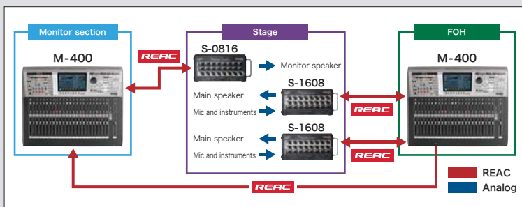
If you take advantage of the three REAC ports and the flexible REAC network, you create a large scale FOH and monitoring system with simple wiring using two M-400s.
