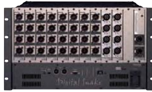
[I/O modular rack] S-4000S-0832
