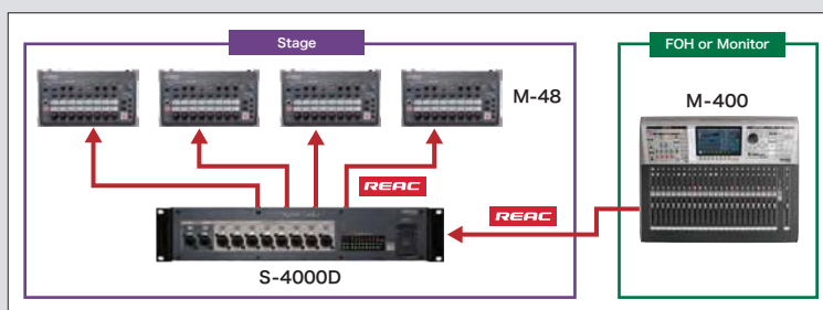
The diagram above shows an example of an M-400 setup with a Personal Mixing System. The S-4000D splitter can send power to the M-48s and is connected via a CAT5e cable. Up to eight units can be connected to a single S-4000D.
