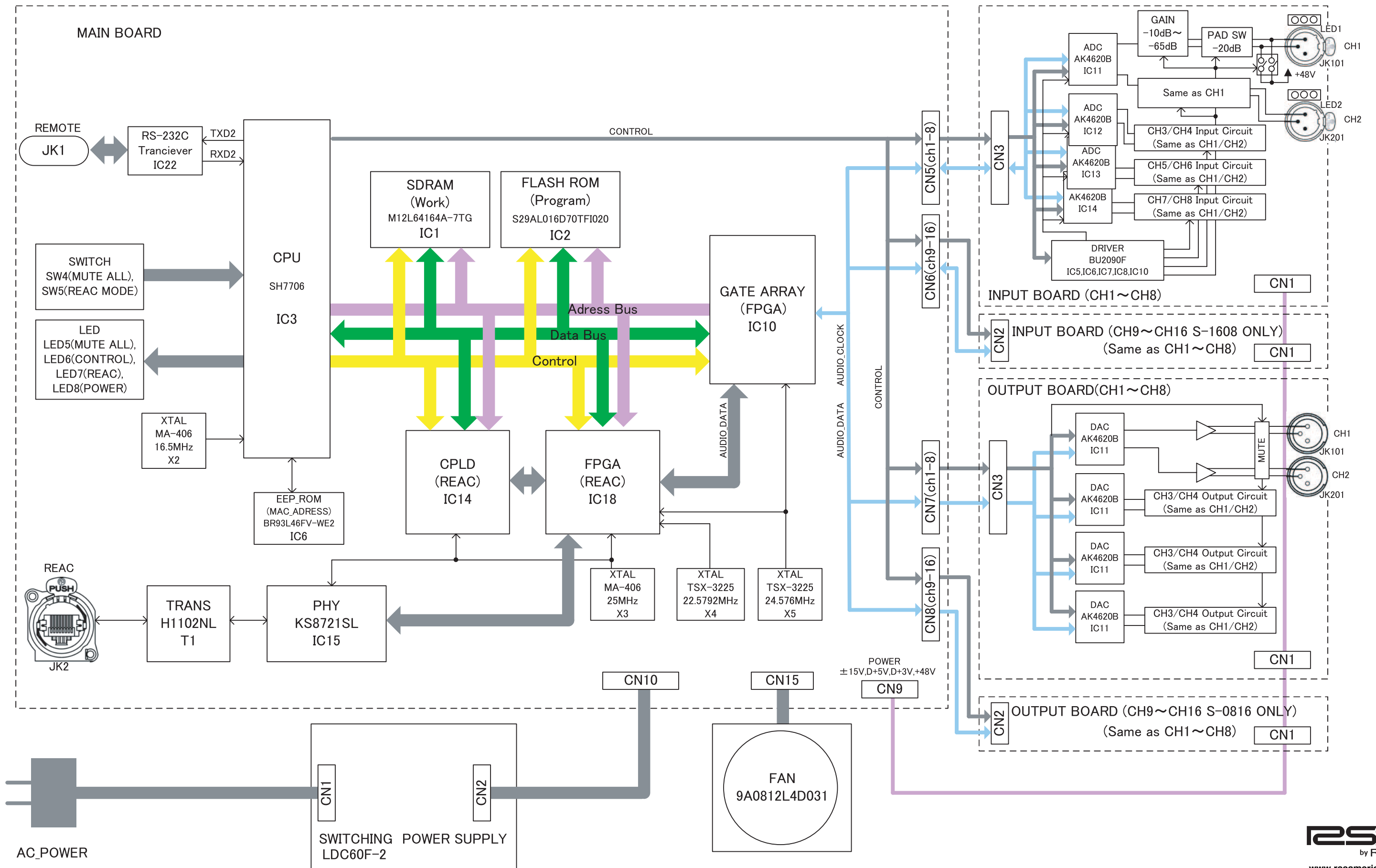
S1608/0816 BLOCK DIGRAM
